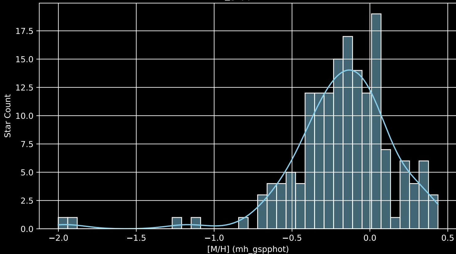
APOGEE DR17 Field: [273-30-O_TESS [M/H] (mh_gspphot) (n= 165)
