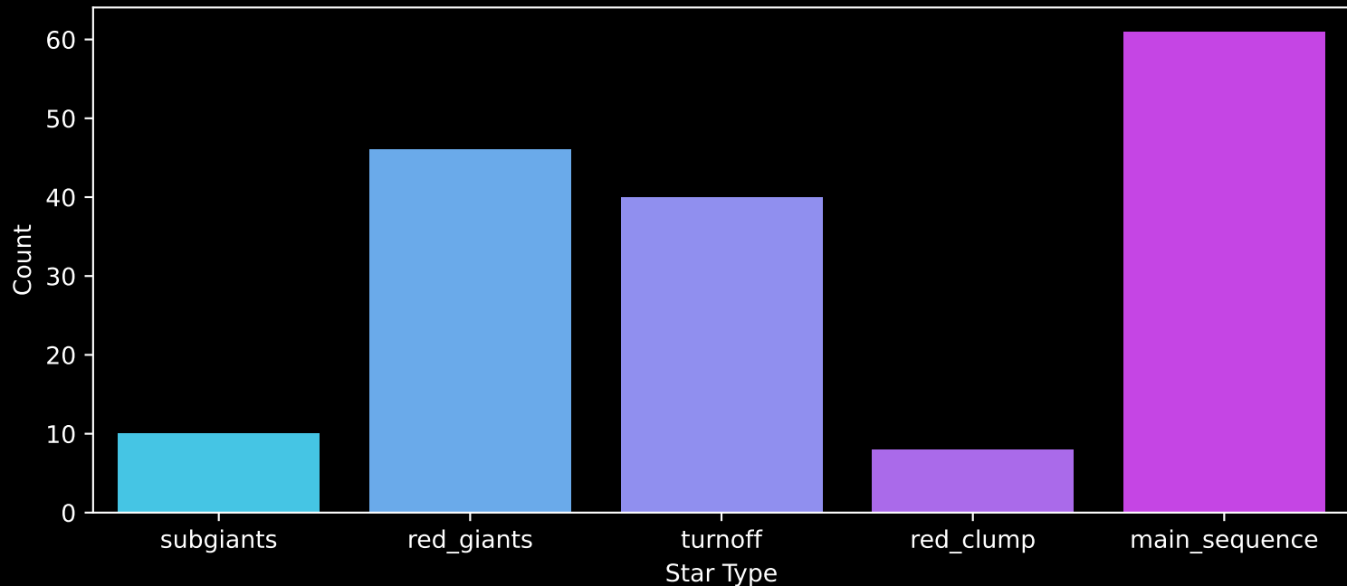
APOGEE DR17 Field: [273-30-O_TESS] Count plot of Star Type
