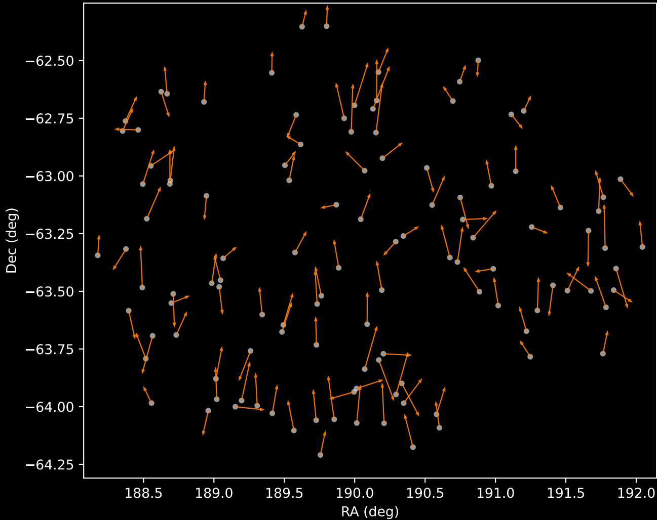
APOGEE DR17 Cluster 2 Proper Motion Vectors (n=116)
