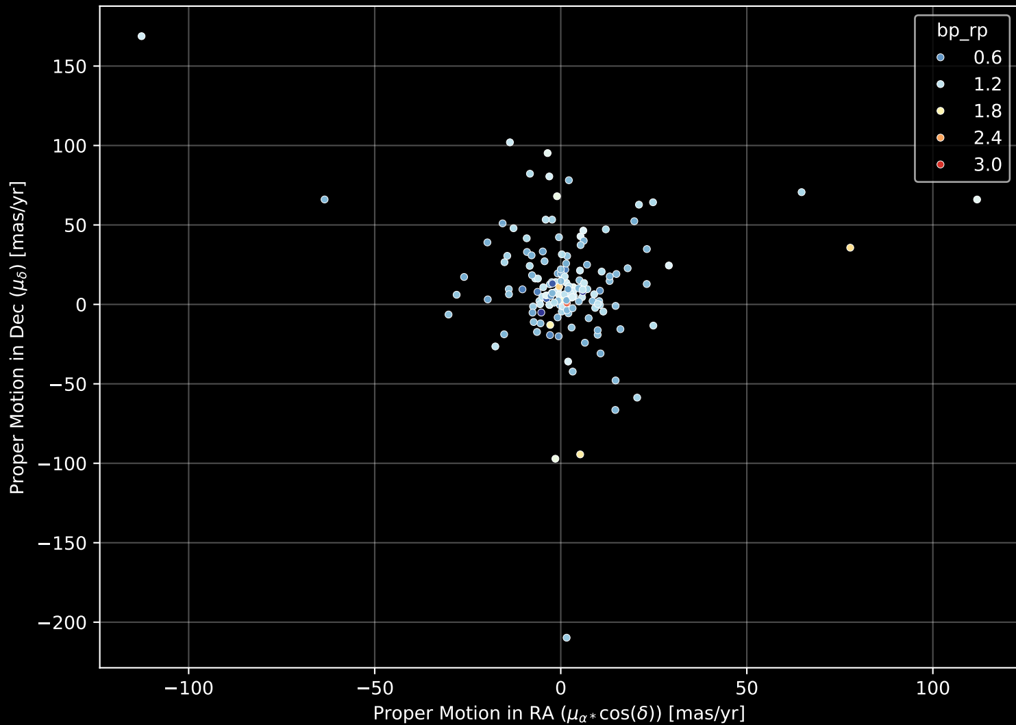
APOGEE DR17 Field: [273-30-O_TESS] Proper Motion Diagram (n= 165)
