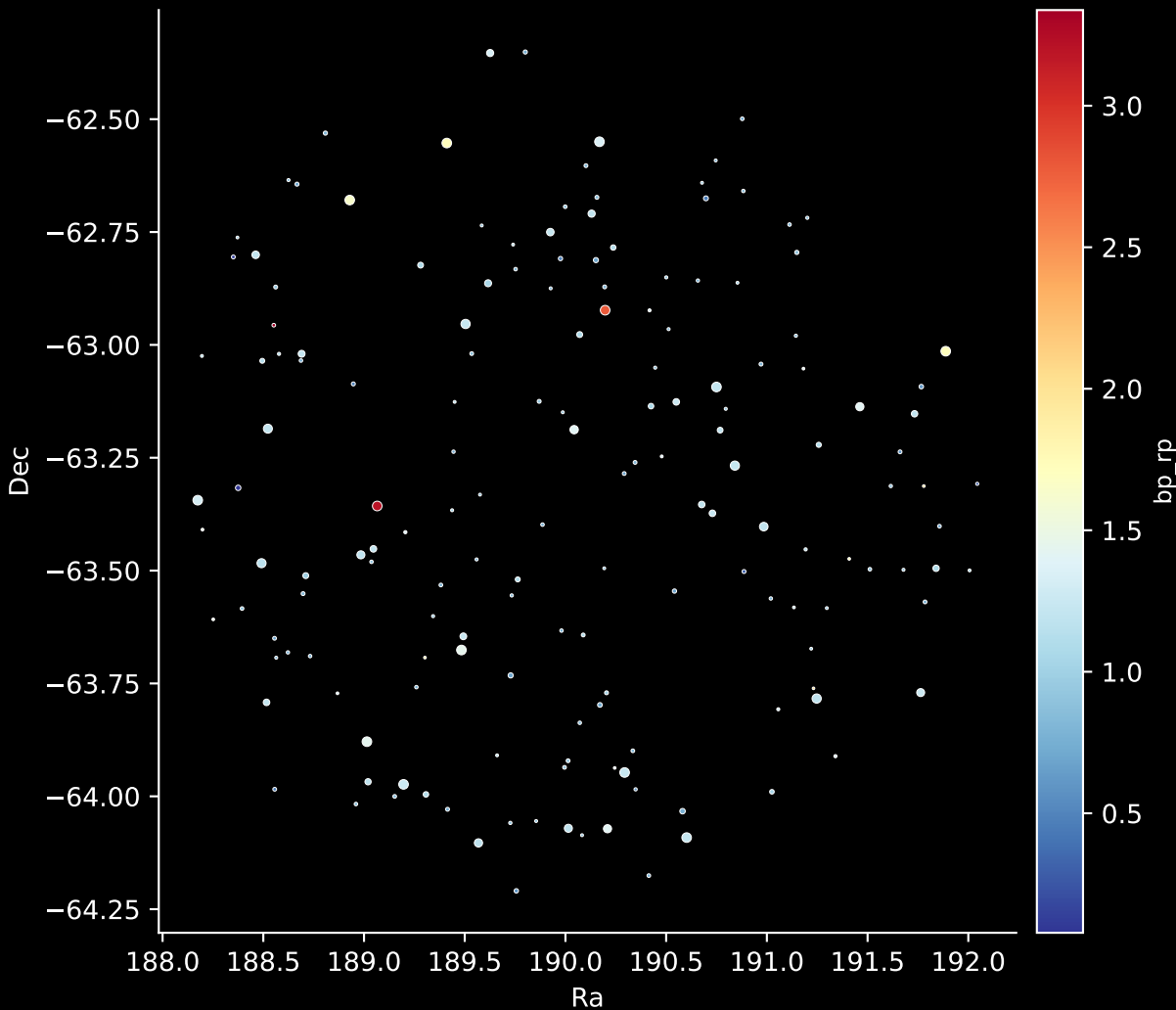
APOGEE DR17 Field: [273-30-O_TESS] Stars: 165
