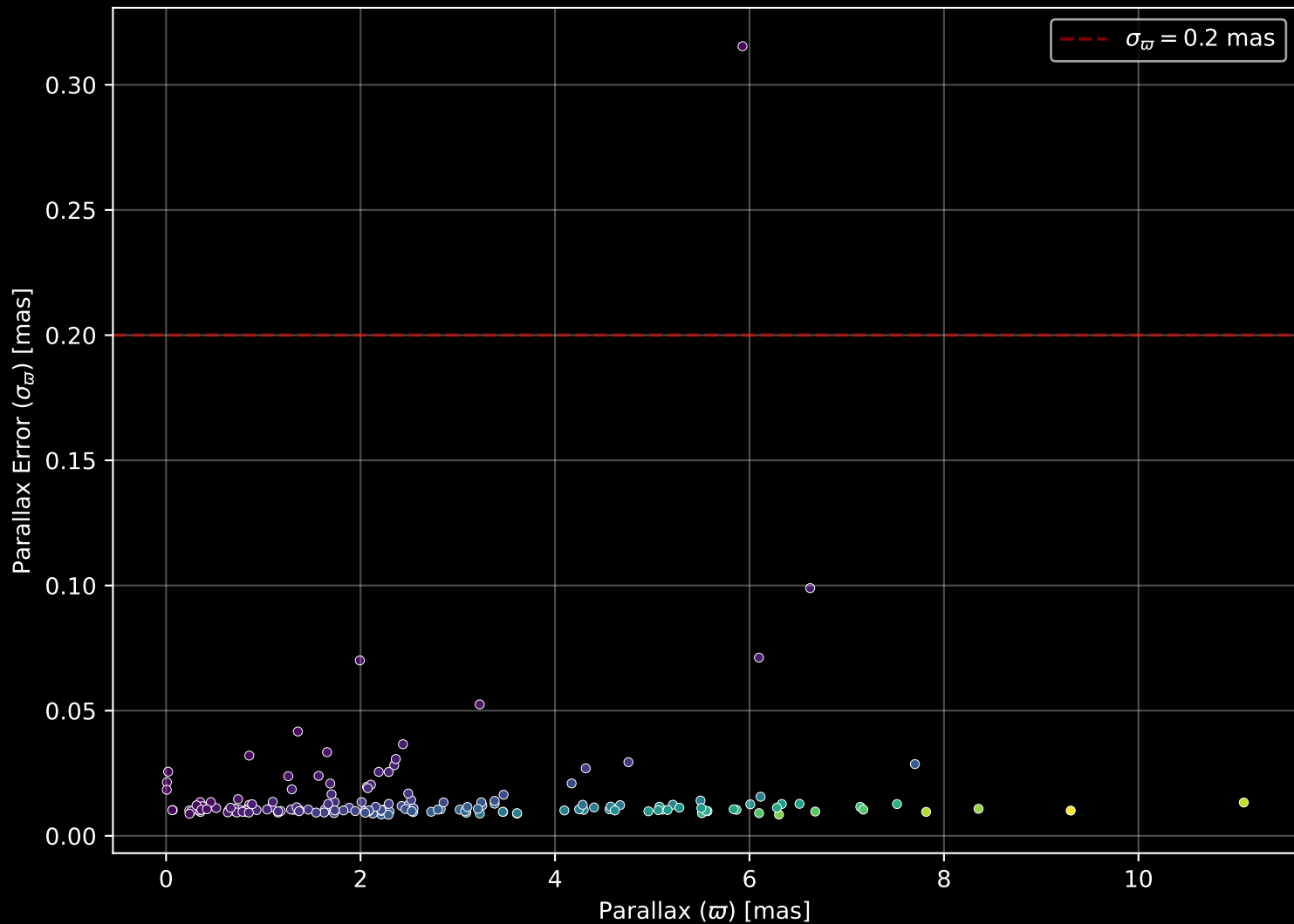
APOGEE DR17 Field: [273-30-O_TESS] Parallax Quality (n= 165)
