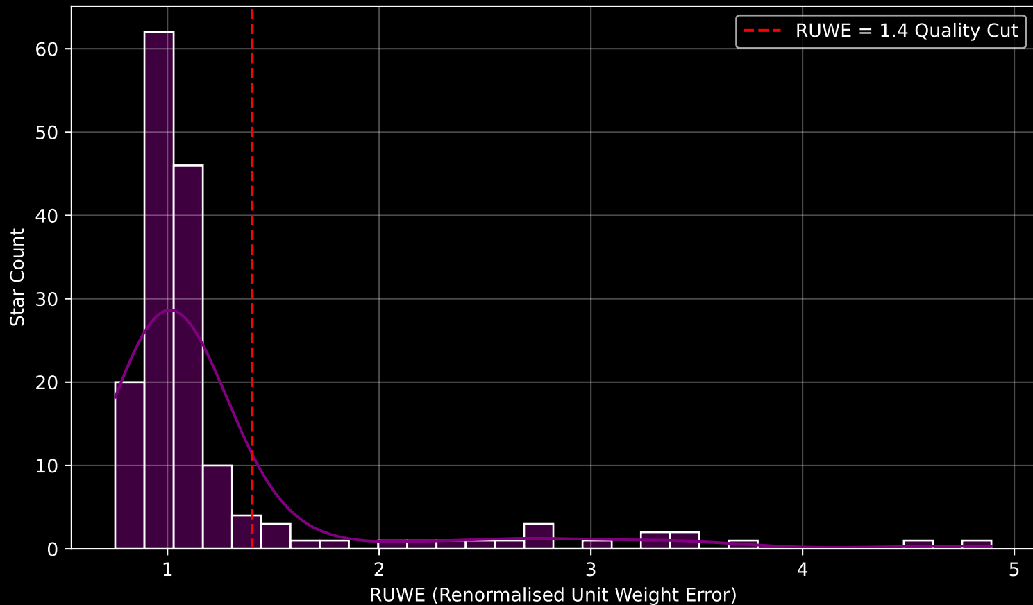
GAPOGEE DR17 Field [273-30-O_TESS] RUWE Distribution (n= 163)
